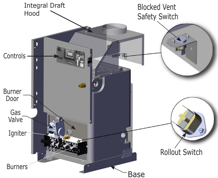
FIGURE 2 - BOILER FLUE GAS PASSAGEWAYS
