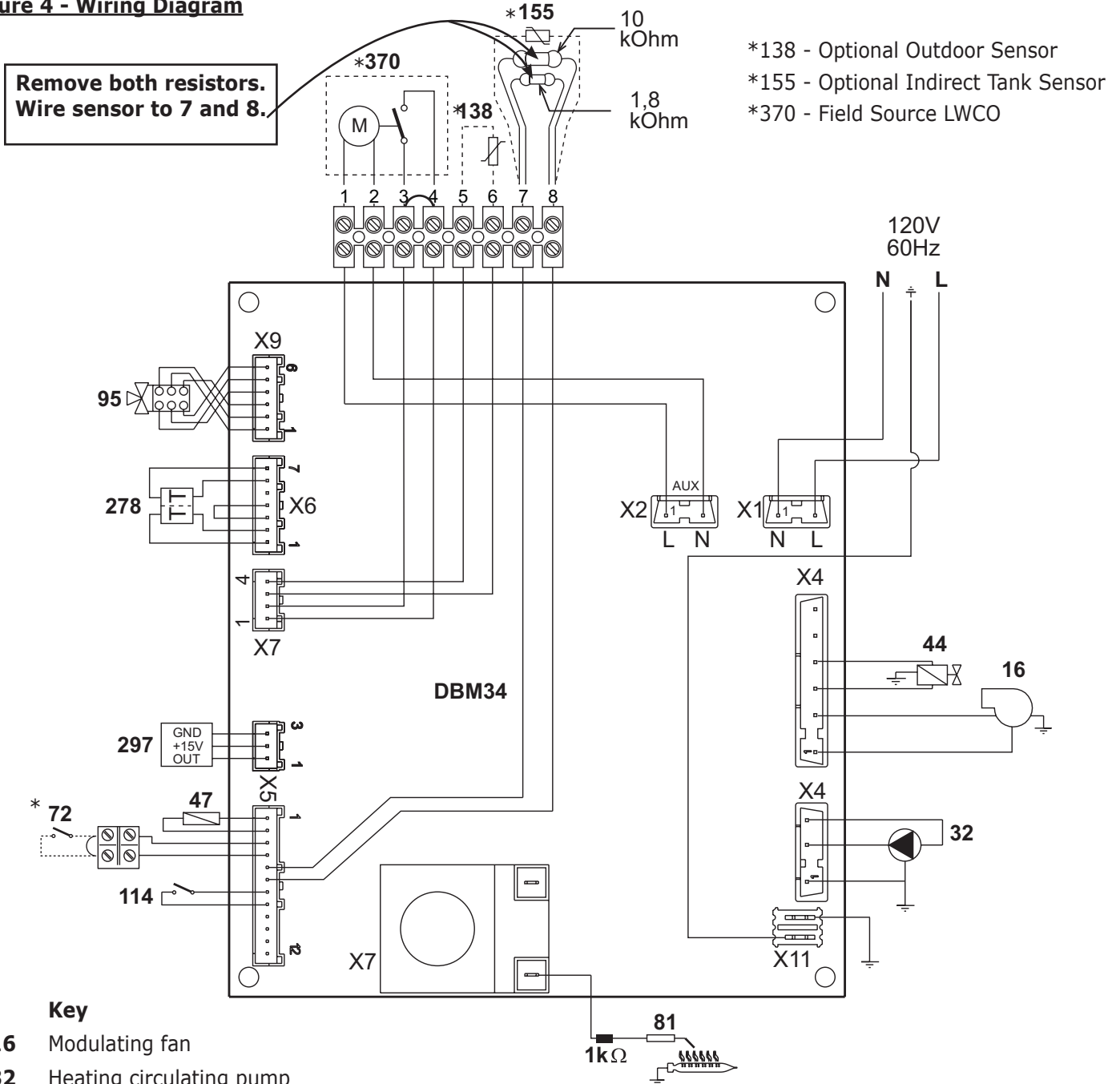
Figure 4 - Wiring Diagram
